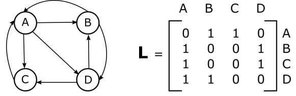
Fig. 3. Example graph with adjacency matrix: the edge j \rightarrow i here means that j refers to i (PageRank) or that j follows i , i.e. \mathbf{1}_{\{j \in \mathcal{F}^{(i)}\}} = \mathbf{1}_{\{i \in \mathcal{L}^{(j)}\}} = 1 (Newsfeed), and we set \ell_{i,j} = 1 in the leader matrix \mathbf{L} .
