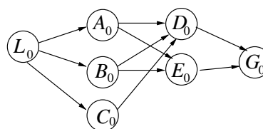
Fig. 8. An example of several diamonds caused by load balancing. For clarity, we omit the probe packets.
