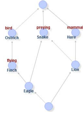
Figure 1. Generated concept lattice for the animal's context in table 1.
